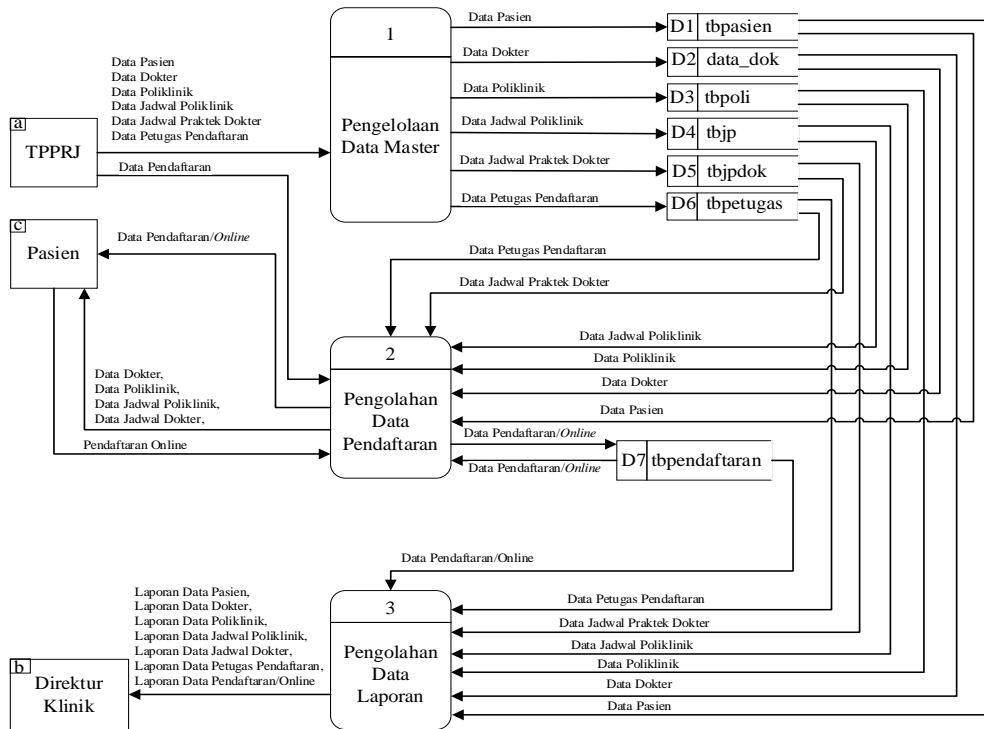
Gambar 2 DFD Level 0
