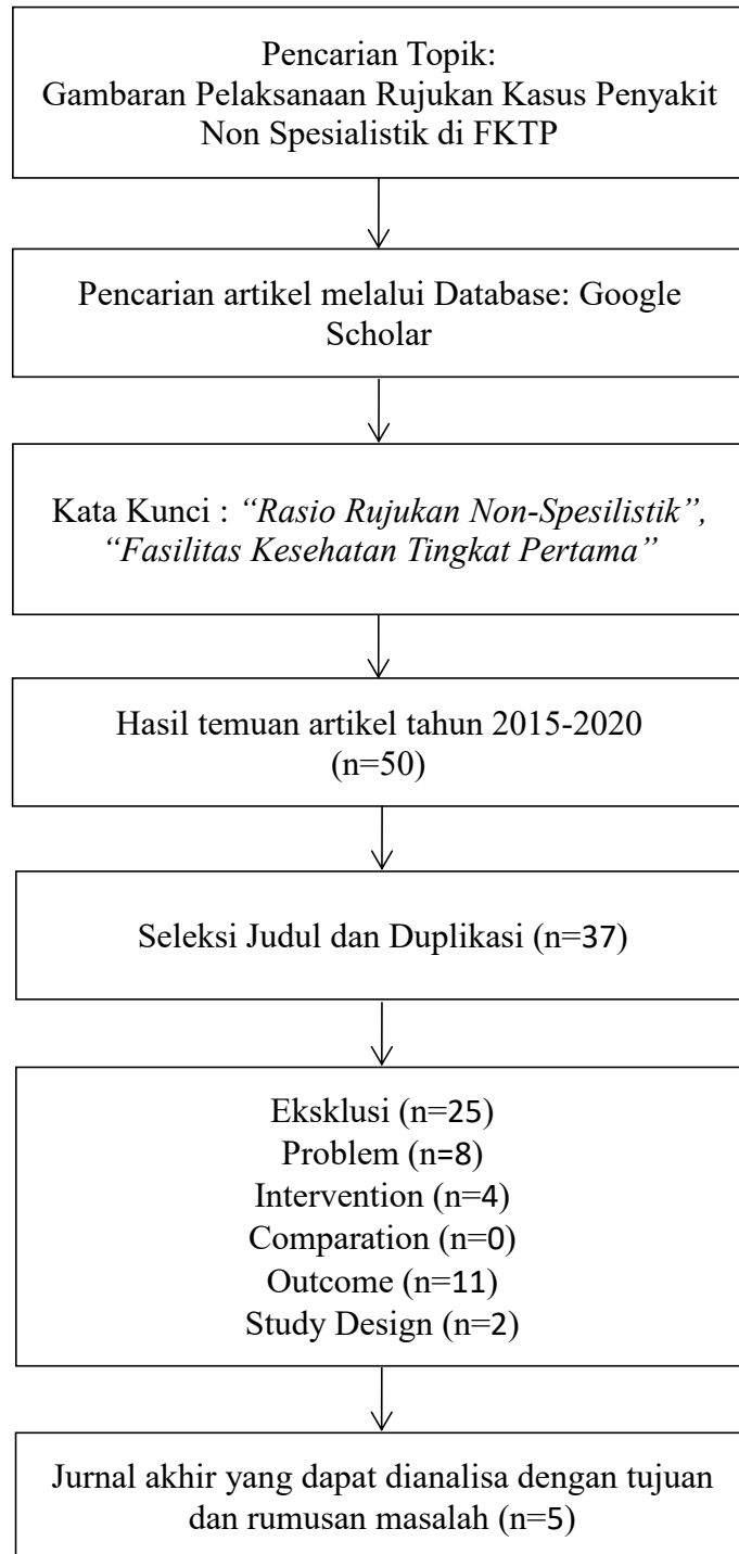
Gambar 3.1 Diagram Alur
